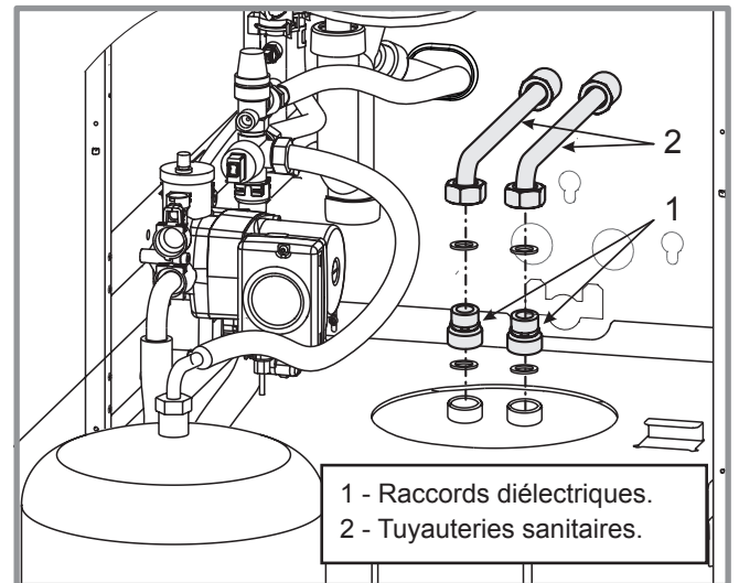
figure 20 - Tuyauteries sanitaires (perfinox condens duo)
