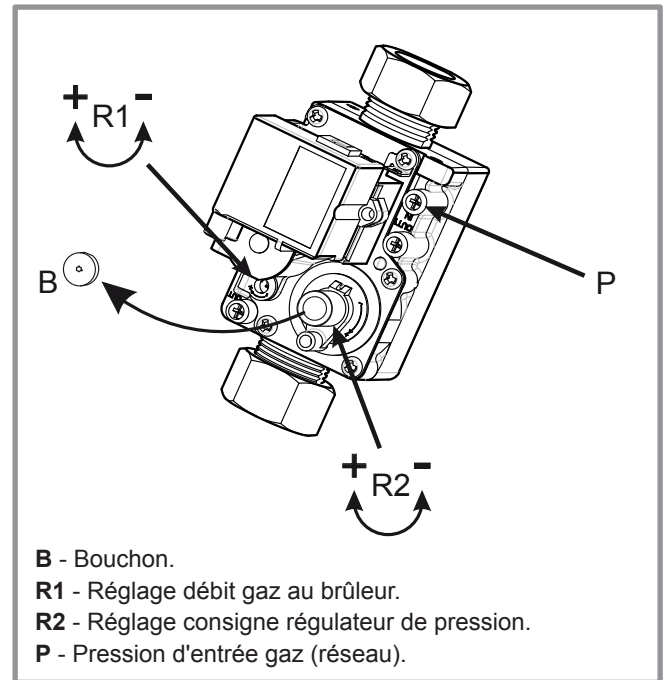
figure 36 - Vanne gaz
