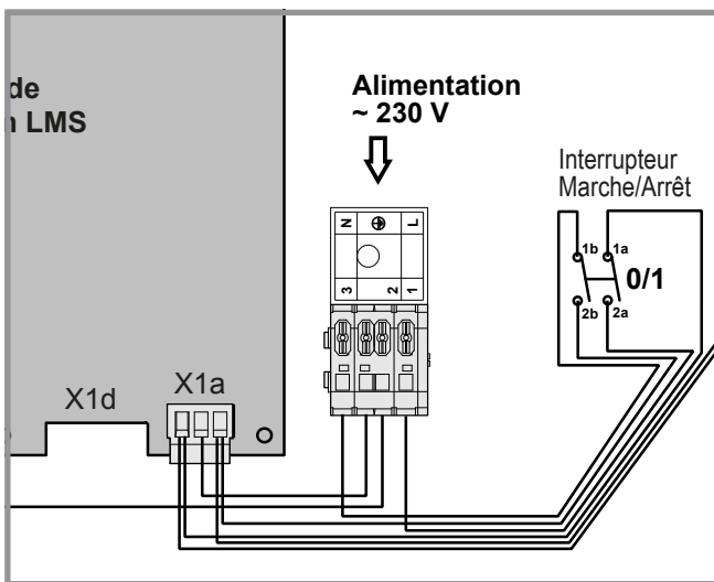
figure 28 - Raccordement alimentation
