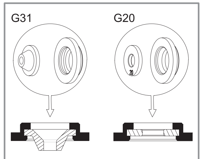
figure 23 - Diaphragme vanne gaz
