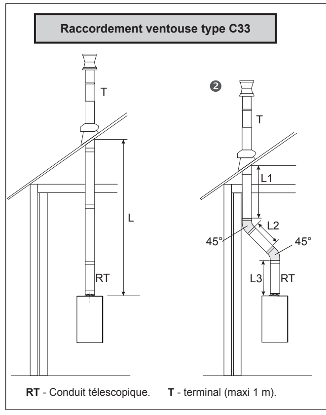
figure 14 - Possibilités de raccordement (type C33, C93)
