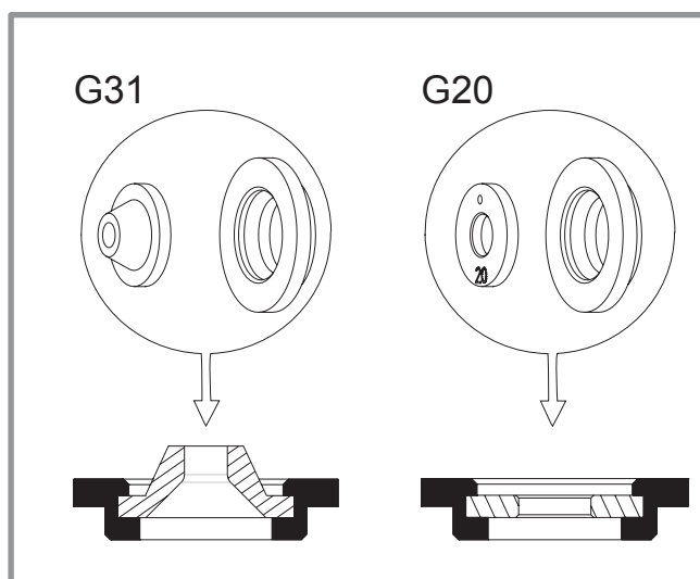
figure 12 - Diaphragme vanne gaz
