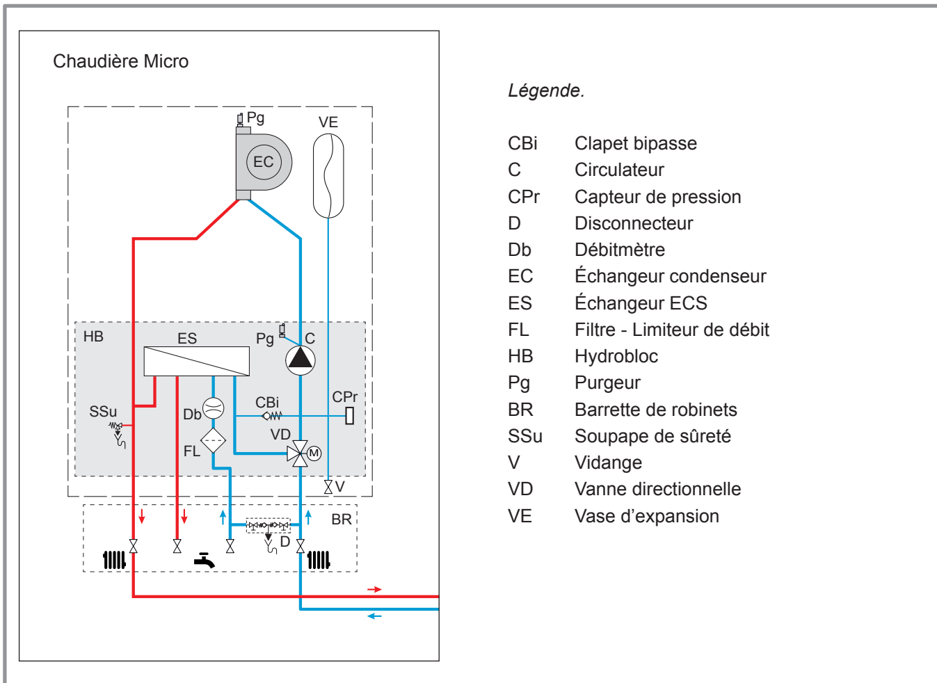
figure 7 - Principe hydraulique
