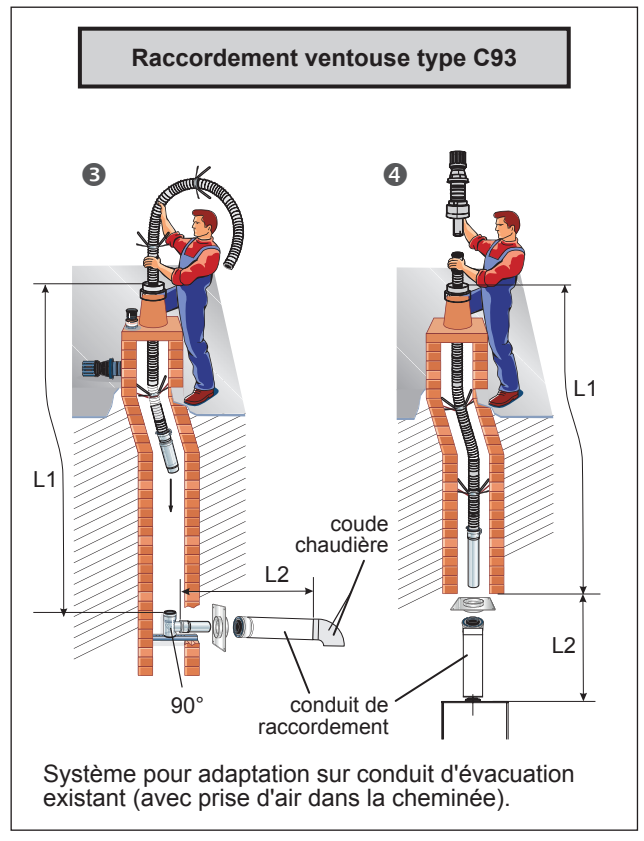
figure 14 - Possibilités de raccordement (type C33, C93)
