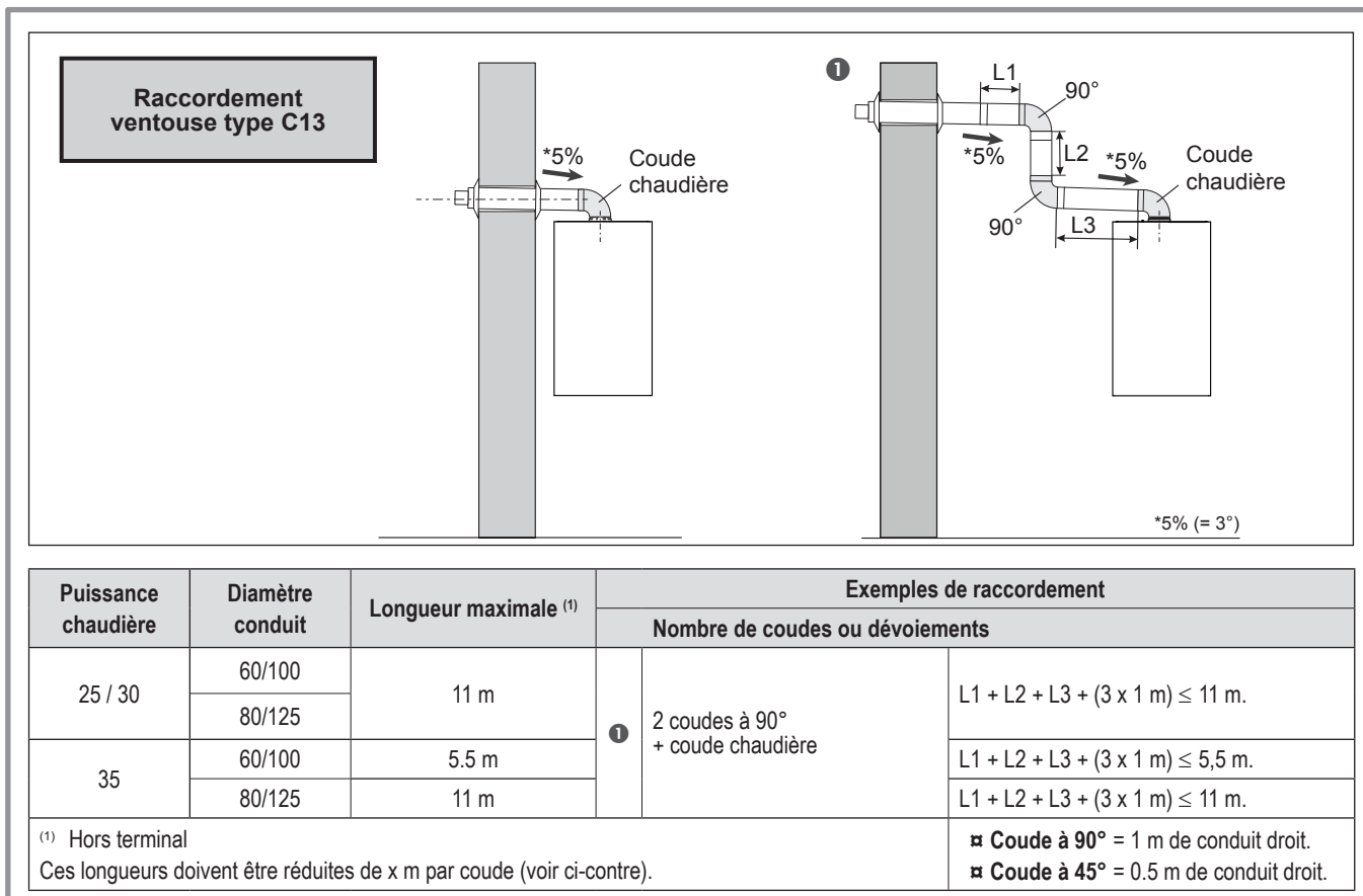
figure 13 - Possibilités de raccordement (type C13)
