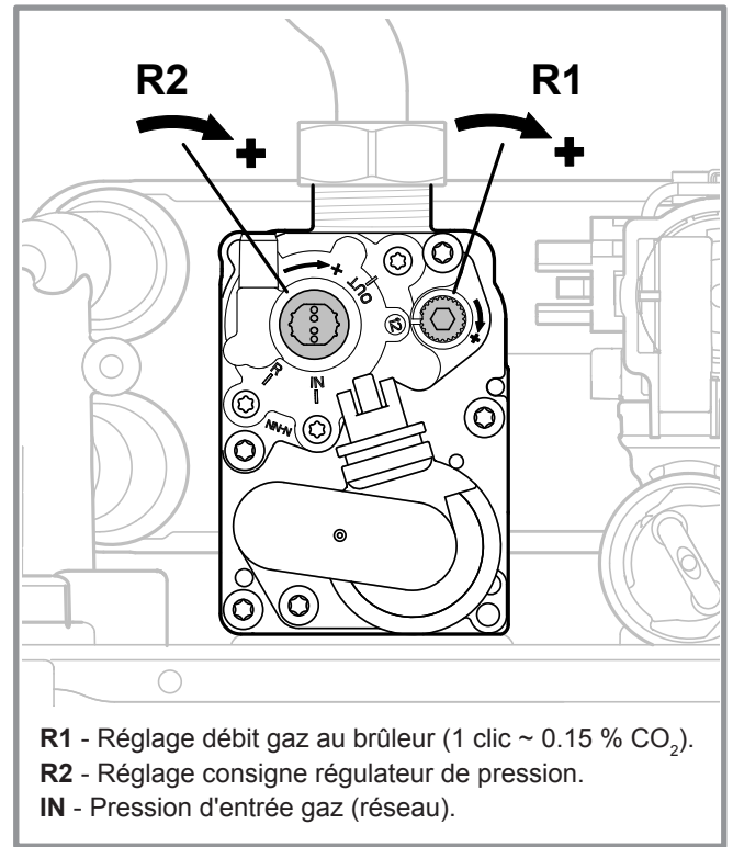
figure 23 - Vanne gaz
